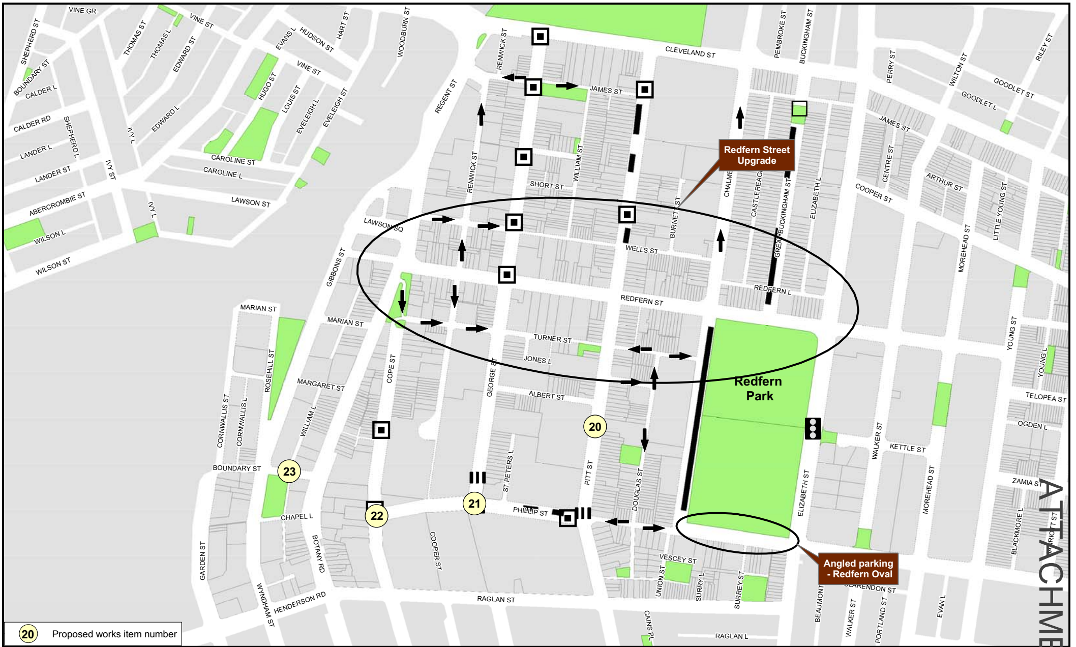
Figure 7.2 Proposed Traffic Management West Redfern 30/3/07
